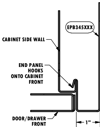
SECTION BP-BP FRONT DETAIL
