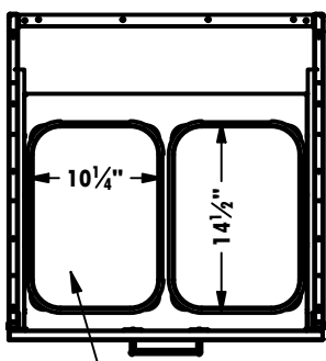
SECTION AF-AF SCALE 3/4" = 12"
